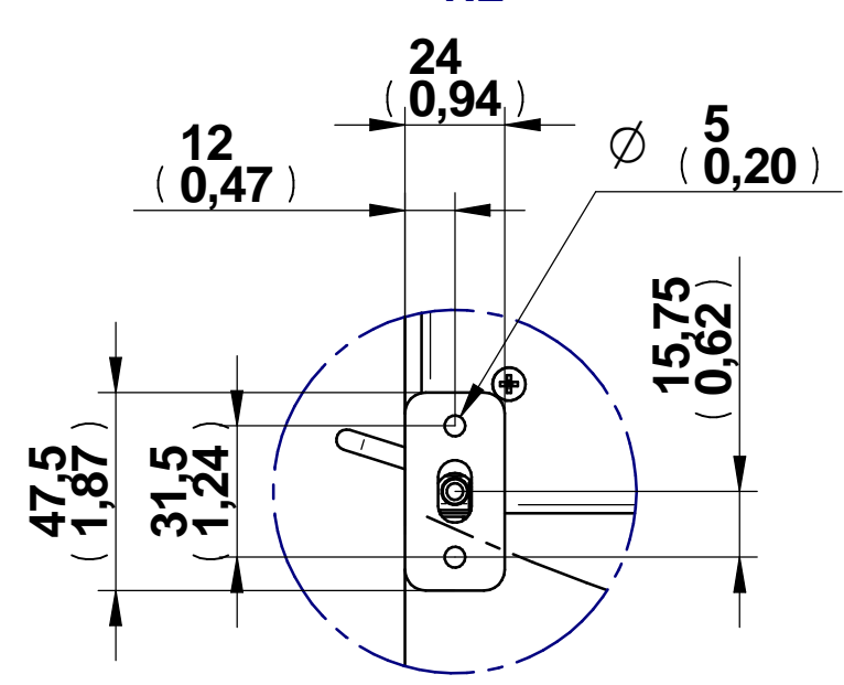
GIMBLE LOCK PLATE DETAIL 1:2
